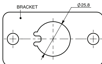
Figure 3: Secure Bracket
